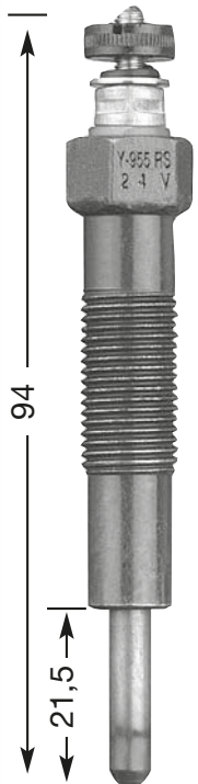
Y-955 RS M 12 x 1.25 14 Hex 24 V
