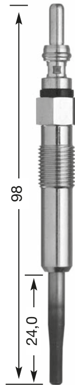
Y1035 AS M 10 x 1.0 10 Hex 4,4 V DP 77
