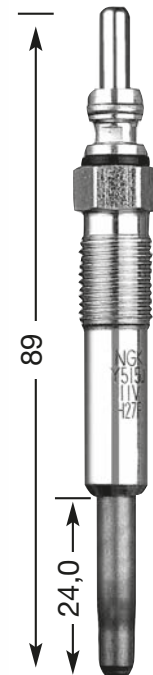
Y-515 J M 10 x 1.0 10 Hex 11 V DP 18
