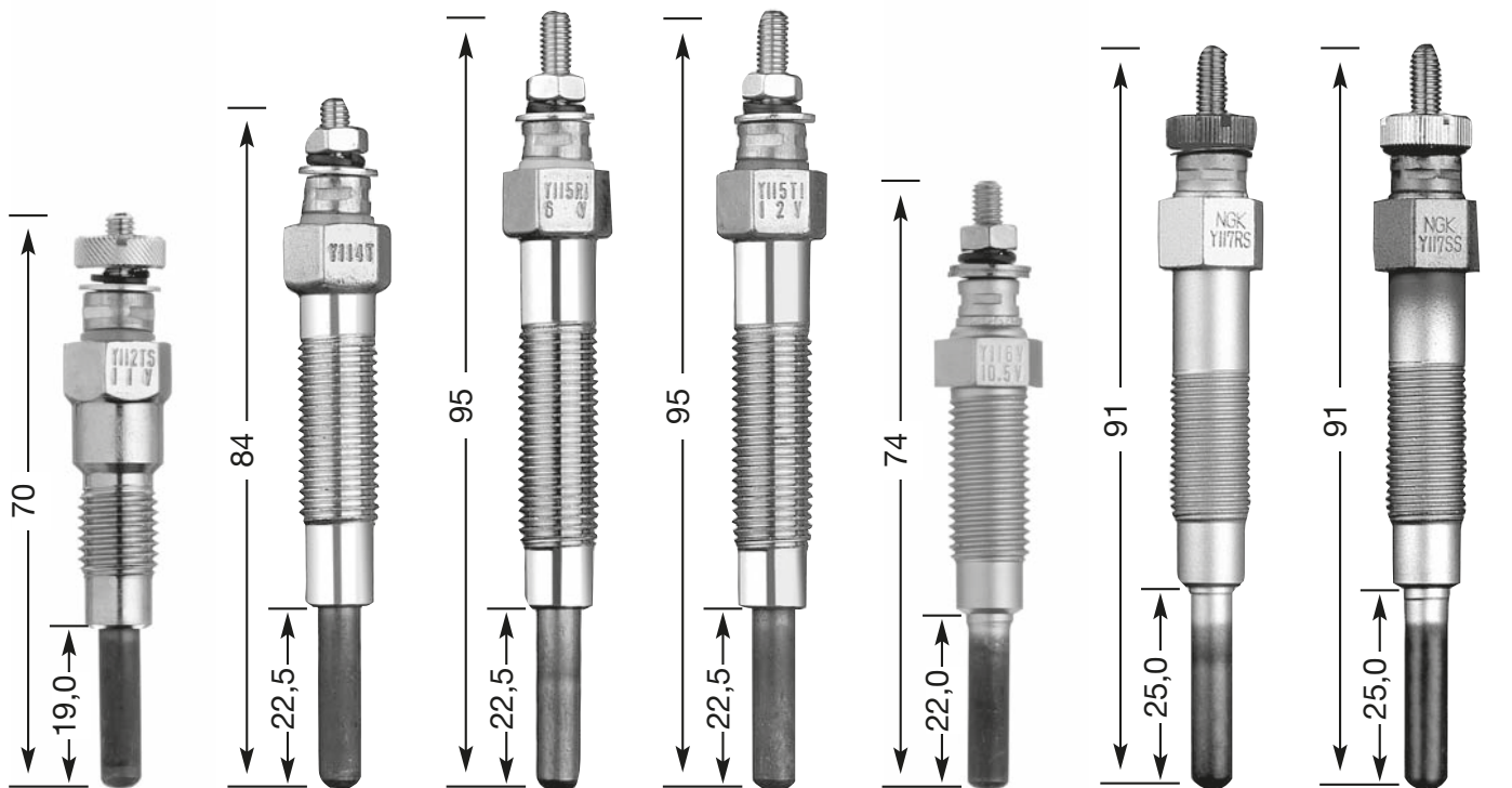
Y-112 TS M 10 x 1.25 12 Hex 11 V
