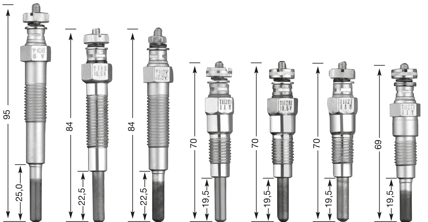
Y-108 M 10 x 1.25 12 Hex 8 V
