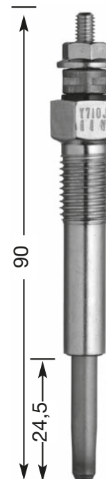
Y-710 J M 10 x 1.25 12 Hex 11 V
